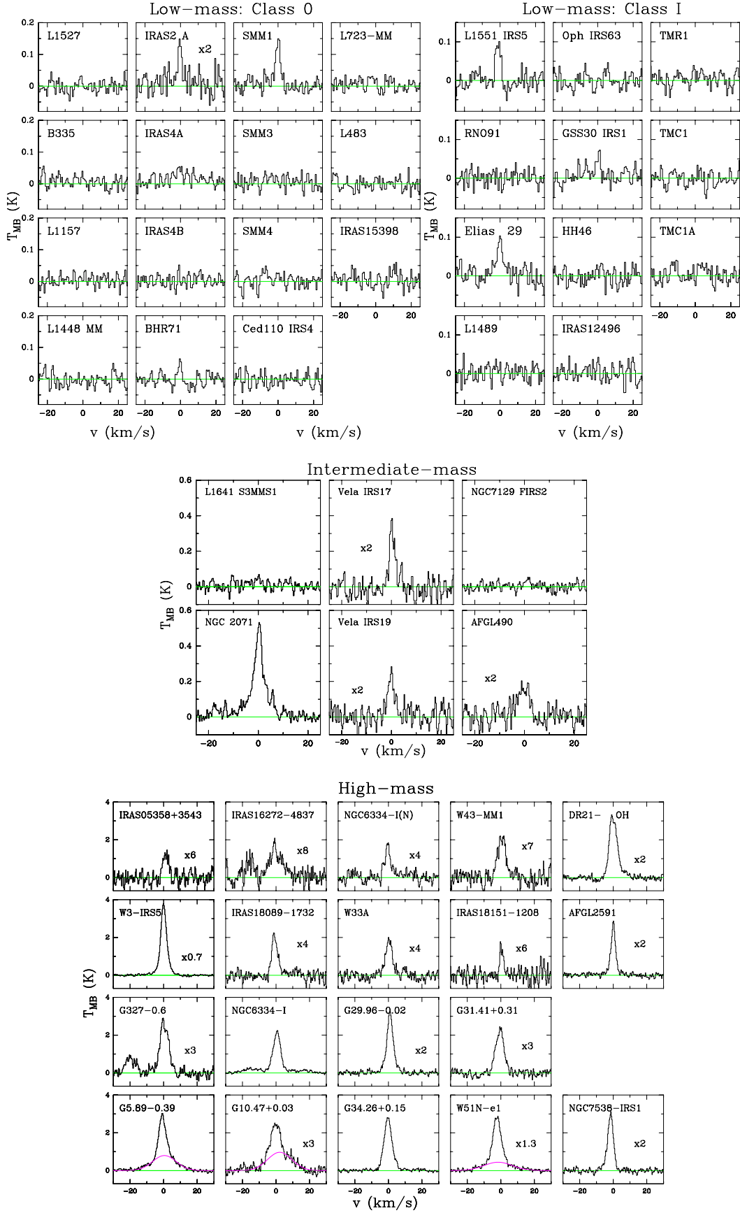
Fig. A.4. Same as Fig. A.1 but for the C^{18}O J = 9-8 spectra from the low-, intermediate- and high-mass YSOs. The high-mass objects are organised according to their evolutionary stage, as is explained in Fig. A.2.
