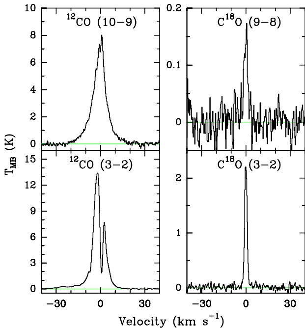
Fig. B.1. Comparison between high- J HIFI and low- J JCMT spectra for the low-mass source Ser SMM1. ^{12}\text{CO} J = 10-9 spectra (left-top) and \text{C}^{18}\text{O} J = 9-8 line (right-top) observed with HIFI and for the ^{12}\text{CO} J = 3-2 and \text{C}^{18}\text{O} J = 3-2 lines (left-bottom and right-bottom respectively) observed with JCMT. The spectra have been resampled to 0.27 \text{ km s}^{-1} and shifted to zero velocity. The green line indicates the baseline subtraction.
