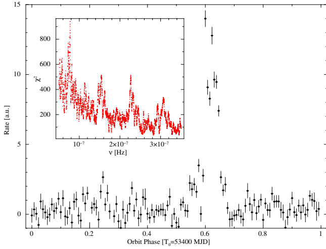
Fig. 2. Folded Swift /BAT light curve (15–150 keV) of RXJ0440.9+4431 at the best determined orbital period, (150.0 \pm 0.2) days. The inset shows the periodogram obtained from the epoch folding technique applied to the Swift /BAT light curve.
