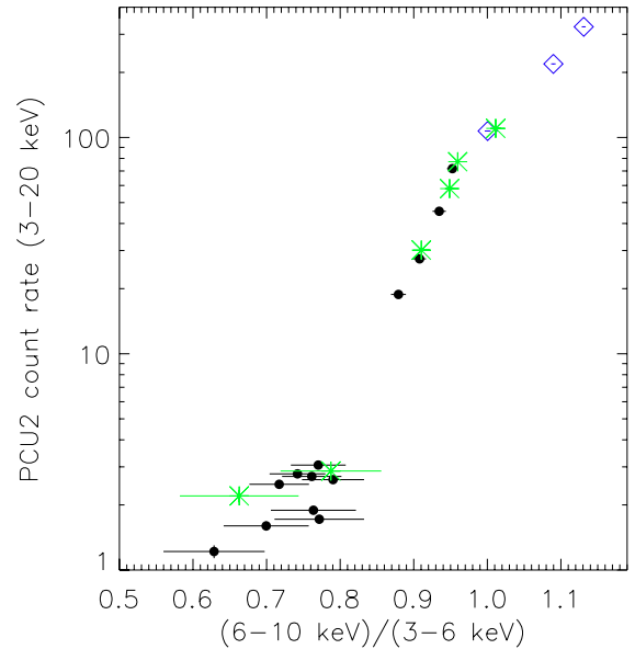
Fig. 5. Hardness-intensity diagram of all the available PCA observation of RX J0440.9+4431. Different symbols refer to different outbursts: diamonds are for the outburst in April 2010 (MJD 55 292–55 301), stars for the outburst of September 2010 (MJD 55 447–55 450), and black dots for the outburst of February 2011 (MJD 55 594–55 606).
