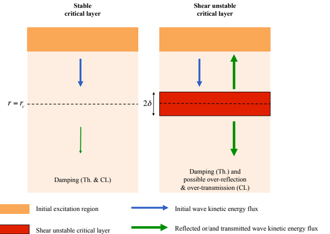
Fig. 5. Two configurations in a low-mass star with an external convective envelope. Left : the case of a stable critical layer (CL) where IGW are damped. Right : the case of an unstable critical layer where IGW can be over-reflected/transmitted.
