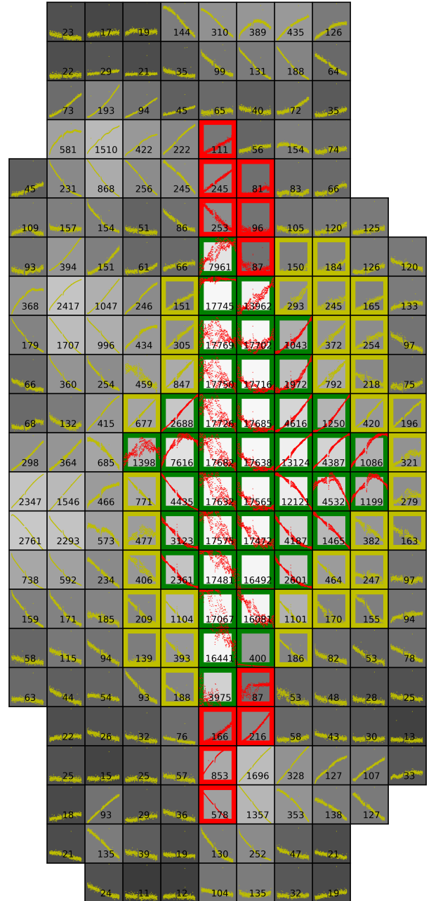
Fig. 9. Custom pixel mask for the Q8 data of KIC 4930889. Individual pixel-level light curves are plotted for each pixel that was downloaded from the spacecraft. The numerical values and the background colour indicate the flux levels in each pixel. The pixels with green and red borders were used to extract the standard Kepler light curves. We added yellow pixels (significant signal is present) and removed red pixels (non-significant signal or contamination from nearby stars) in our custom mask for the light curve extraction. This results in a light curve with significantly less instrumental effects and/or contamination than the standard extraction.
