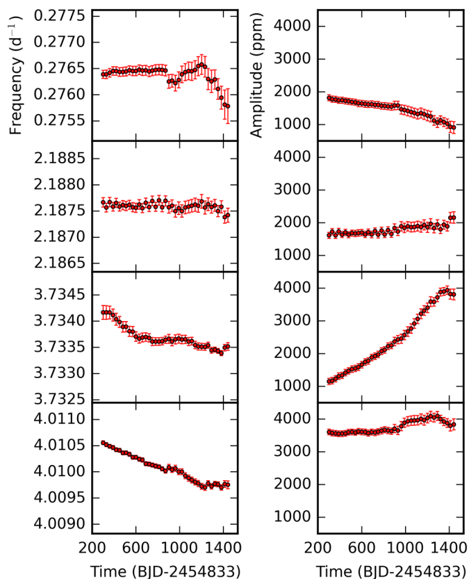
Fig. 22. Frequency (left panels) and amplitude (right panels) variations of the four strongest pulsation modes traced from the STFT of KIC 11971405, which was calculated using 360 d wide windows that were stepped with 30 d.
