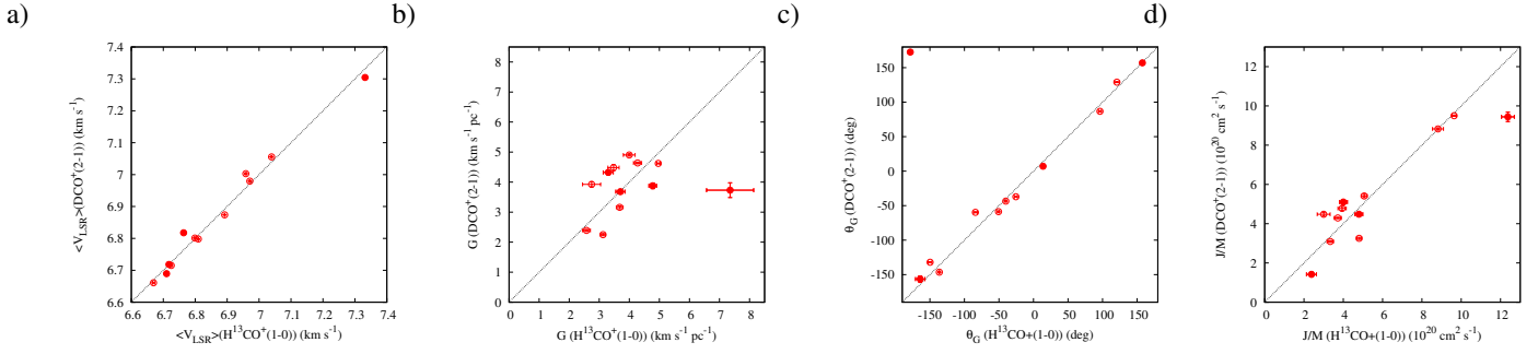
Fig. B.3. DCO + (2–1) compared to H 13 CO + (1–0): a ) average velocity across the core; b ) total velocity gradient; c ) position angle of the total velocity gradient; d ) specific angular momentum. Open circles show starless cores and filled circles show protostellar cores. For the comparison, all maps are convolved to the largest beam of 29.9'' with Nyquist spacing and only the area that contains both H 13 CO + (1–0) and DCO + (2–1) emission is used.
