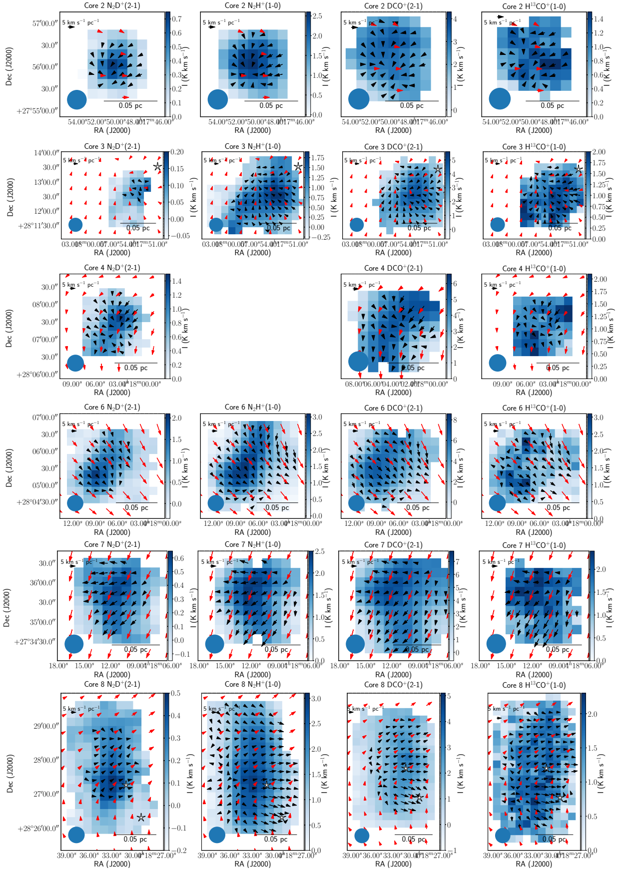
Fig. B.5. V_{\text{LSR}} local gradients of the N_2D^+(2-1) , N_2H^+(1-0) , DCO^+(2-1) , and H^{13}CO^+(1-0) lines across the cores (black arrows) and V_{\text{LSR}} local gradients of the C^{18}O(1-0) line from Hacar et al. (2013; red arrows). The scale of the C^{18}O(1-0) gradients is 2.5 times larger than the scale indicated in the figures. The colour scale shows integrated intensities of corresponding species across the cores. Stars show the positions of YSOs from Rebull et al. (2010): black stars indicate young, flat and Class I objects, white stars indicate more evolved, Class II and III objects.
