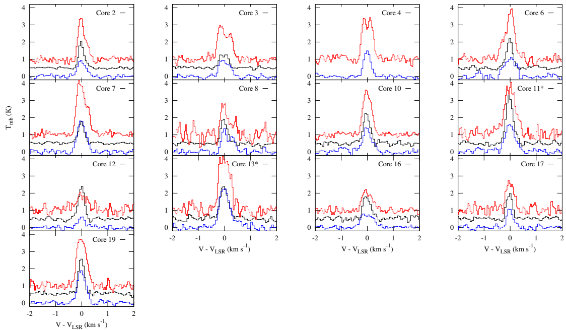
Fig. A.5. Spectra of the isolated components of N_2H^+(1-0) (black), DCO^+(2-1) (red), and H^{13}CO^+(1-0) (blue) towards the N_2H^+(1-0) emission peaks. For convenient comparison, the DCO^+(2-1) spectra are shifted up by 1 K and the N_2H^+(1-0) spectra are shifted up by 0.5 K. The cores with an asterisk (*) near the title contain embedded protostars.
