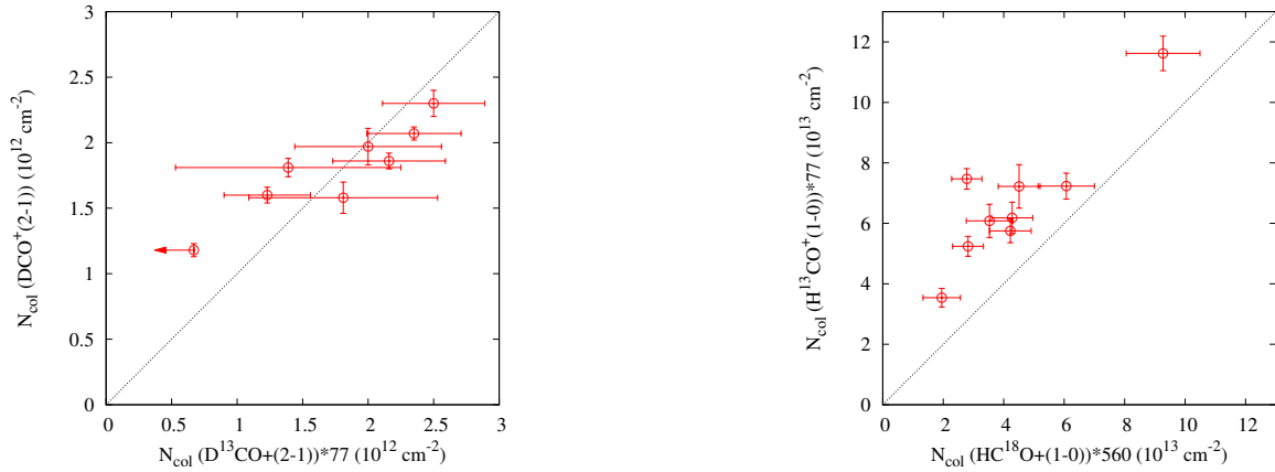
Fig. A.7. Comparison of the column densities of \text{DCO}^+ (left panel) and \text{HCO}^+ (right panel) towards the \text{DCO}^+(2-1) emission peaks obtained with an assumption of optically thin lines. The dotted lines show one-to-one correlations.
