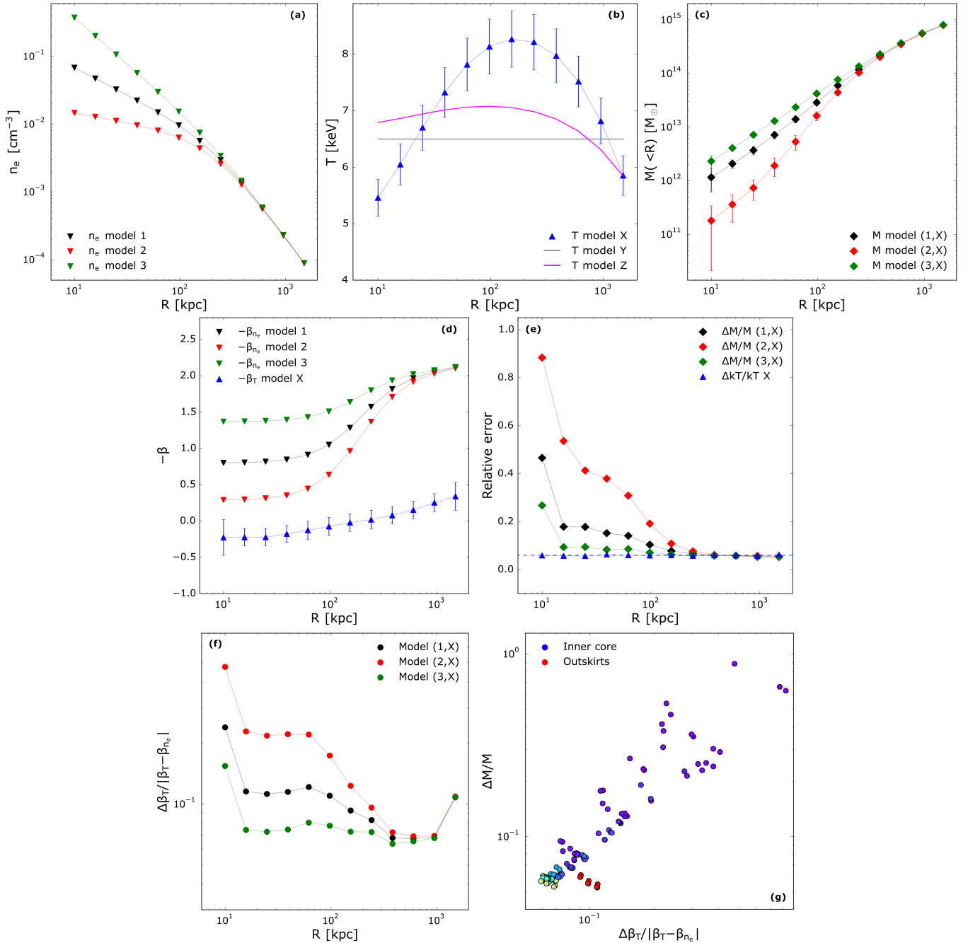
Fig. C.1. Panel a: density profiles generated using the parametric model of Vikhlinin et al. (2006). The errors are set to 0. Panel b: temperature profiles generated using the parametric model of Vikhlinin et al. (2006). The relative error on each bin is fixed to 6%. For clarity, bins and corresponding errors are reported only for “T model X”. We report only the shape form of “T model Y” and “T model Z” with solid grey and magenta lines, respectively. Panel c: hydrostatic mass profiles derived from the three density profiles and from the temperature profile “T model X” shown in panel a and b, respectively, using the FP method. Panel d: \beta is defined as the logarithmic derivative of the density and temperature, namely \beta(n_e) and \beta(kT) , with respect to the logarithm of the radius, \beta \equiv \partial \ln x / \partial \ln r . The errors of \beta(kT) are derived via a Monte-Carlo procedure. Panel e: temperature and mass profile relative errors as a function of the radius. The dotted line represents the 6% relative error. The mass profiles are computed using the three density profiles and the “T model X”. Panel f: ratio between the error of \beta(kT) and the distance D between \beta(n_e) and \beta(kT) , the distance being defined as D \equiv |\beta(kT) - \beta(n_e)| . Panel g: mass profile relative errors as a function of the same quantity shown on the y axis of panel f. For this plot, we also included the results using all the temperature profiles. Points are colour-coded in order to clearly identify the inner core (blue points, upper right part of the plot) and the outskirts (red points, lower left part of the plot). For all the panels except panel g: points represent the quantity measured at fixed radial bins. The solid line is showed to guide the eye.
