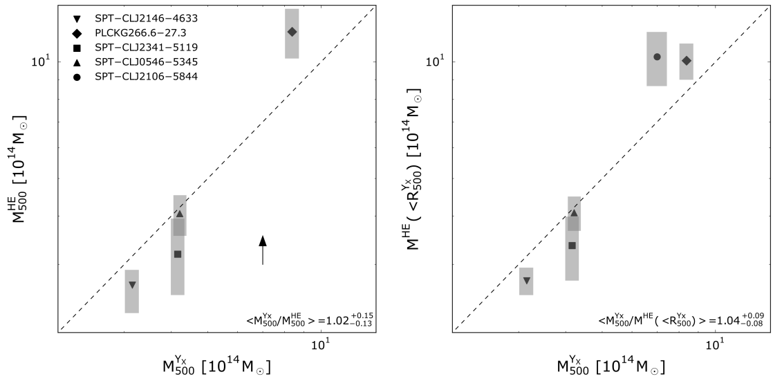
Fig. 5. Left panel: comparison between M_{500}^{\text{Yx}} computed iteratively through the M_{500} - Y_x relation and the hydrostatic mass, M_{500}^{\text{HE}} . The estimates are consistent within the statistical errors. The M_{500}^{\text{HE}} of SPT-CLJ2106-5844 is \sim 3.5 greater than M_{500}^{\text{Yx}} (see Sect. 2.4.2). For this reason, the point is off the scale and its M_{500}^{\text{Yx}} is instead shown with the black arrow. The black dotted line is the 1 : 1 relation. Right panel: same as the left panel, except showing the comparison between M_{500}^{\text{Yx}} and M_{500}^{\text{HE}} (<R_{500}^{\text{Yx}}) . Error-weighted mean ratio and corresponding errors are reported in each panel.
