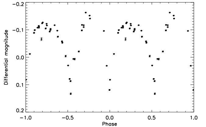
Fig. 8. Light curve for F2. The outlying point with larger uncertainty at phase 0.187 was associated with an incomplete observing run and has been excluded from further analysis.
