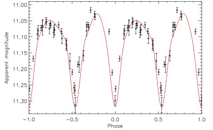
Fig. 12. Light curve for F2 with best-fit (unconstrained) PHOEBE model overlotted in red.
