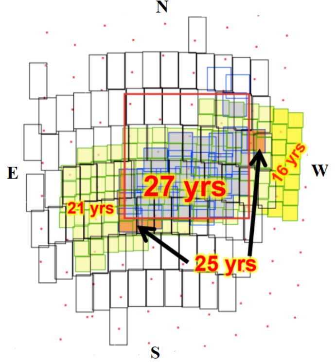
Fig. 2. Fields monitored toward the LMC: EROS 1 plate (large red square), MACHO fields used to measure the optical depth (Alcock et al. 2000b, blue squares), EROS-2 (black rectangles), and OGLE-III (green squares). Red dots show the positions of (a fraction) the OGLE-IV field centers. The gray field contains catalog 1, which has been observed for 27 years. The orange and gray field covers catalog 2, which has been observed for 25 years. Catalog 3 is contained in the light yellow, orange, and gray field, and it has been observed for 21 years. Finally, the combination of all the colored fields contains catalog 4, which has been observed for 16 years.
