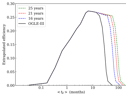
Fig. 3. Conservative extrapolated microlensing detection efficiencies toward the LMC for a combined survey analysis as a function of the event characteristic duration t_E .
