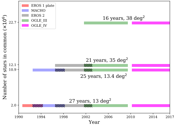
Fig. 1. Catalogs of stars monitored by the different surveys; numbers of stars, field sizes, and observation epochs. Hatched regions show periods in which different surveys overlapped.
