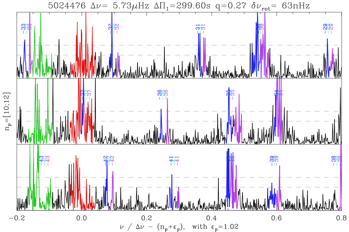
Fig. B.1. Fit of the oscillation pattern of the RGB star KIC 5024476, member of the open cluster NGC 6819. The dim magnitude of the cluster stars explains the low S/N. However, unambiguous doublets are identified all along the mixed-mode spectrum; m = 0 modes are mostly absent and |m| = 1 modes dominate the mixed-mode spectrum, so that a nearly pole-on inclination is not possible. Same style as Fig. 2.
