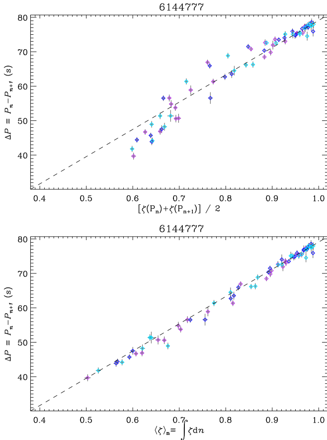
Fig. 4. Period spacings of the RGB star KIC 6144777. Top: plot as a function of the arithmetical mean value (\zeta(v_n) + \zeta(v_{n+1}))/2 . Bottom: plot as a function of the mean value \langle \zeta \rangle_n . The colors code the azimuthal orders, as in Fig. 2; the dashed line indicates the 1:1 relation; 1- \sigma uncertainties on both the spacings and the mean values of \zeta are indicated by vertical and horizontal error bars.
