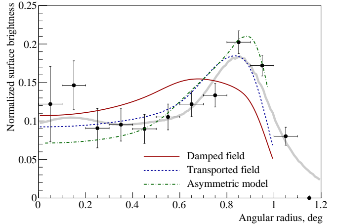
Fig. 7. Simulated radial surface brightness profiles of the gamma-ray emission in the 300 GeV–20 TeV energy range compared to the H.E.S.S. measurements for the northern part of the remnant (Aharonian et al. 2007, black filled circles). Red solid and blue dashed lines show simulated profiles for the spherically symmetric models BOHM_DAMP and BOHM_KOLM, respectively. The radial profile obtained within the asymmetric model discussed in Sect. 4.2 is represented by the green dash-dotted line. This profile is averaged over the azimuth angle for the hemisphere containing the cone of enhanced emission. The thick gray line shows the azimuthally averaged radial profile for the northern part of the SNR extracted from the recently published updated H.E.S.S. excess sky map (H.E.S.S. Collaboration 2018). This sky map is smoothed with a Gaussian function of width 0.08^\circ . All simulated profiles are normalized in the same way as H.E.S.S. measurements in Aharonian et al. (2007).
