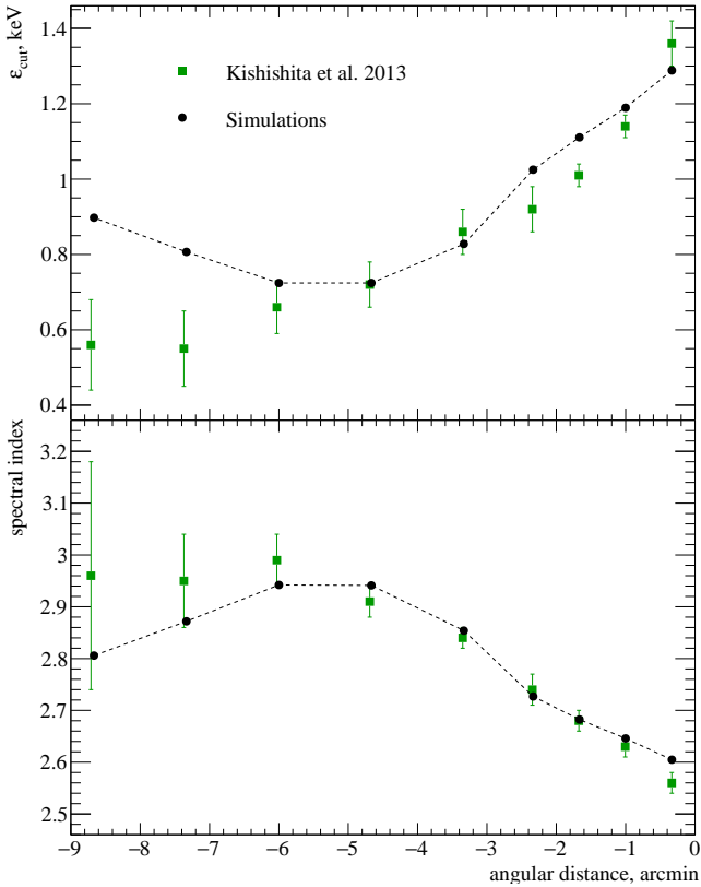
Fig. 8. Simulated cut-off energy ( top panel ) and spectral index ( bottom panel ) of the X-ray spectrum in the filament as a function of the angular distance from the shock compared to the experimental measurements. Simulated distributions are obtained using the asymmetric model described in Sect. 4.2.
