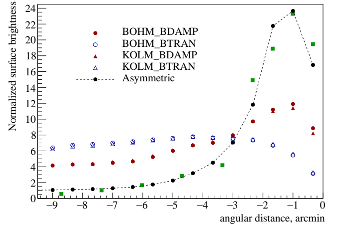
Fig. 5. Simulated projected X-ray radial flux profiles for different models assuming spherical symmetry compared to the experimental measurements (green squares Kishishita et al. 2013). Normalized surface brightness in the energy range 2–10 keV is plotted as a function of the angular distance from the forward shock of the SNR with negative values corresponding to the interior of the remnant. The radial profile obtained within the asymmetric model discussed in Sect. 4.2 is represented by the black filled circles connected with the dashed line.
