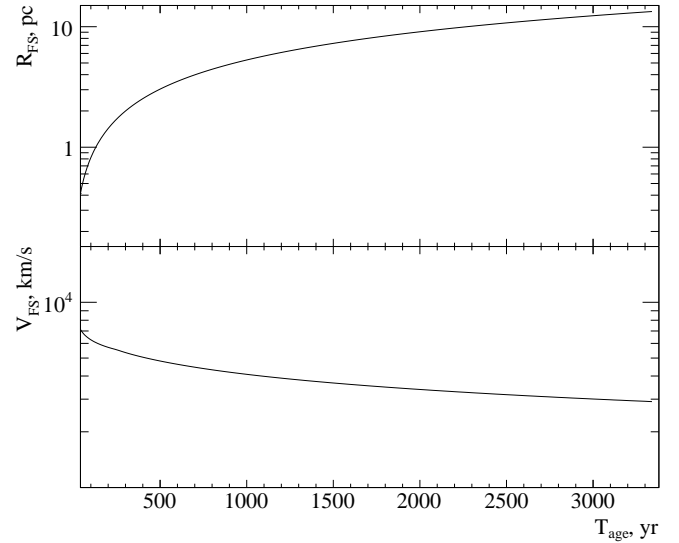
Fig. 1. Time evolution of the forward shock radius ( top panel ) and shock velocity ( bottom panel ) up to the current age as obtained from our hydrodynamic model.
