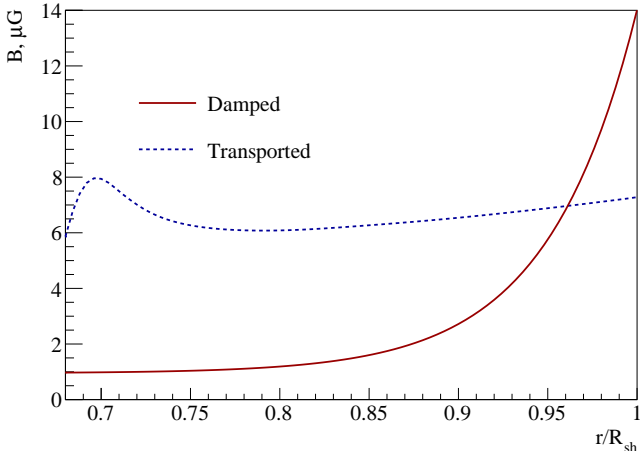
Fig. 2. Magnetic field strength as a function of the normalized radius between the contact discontinuity and the forward shock. Red solid line shows the profile for the magnetic damping scenario and the blue dashed line for the transported magnetic field. Both distributions are shown for the models with the Bohm diffusion coefficient.
