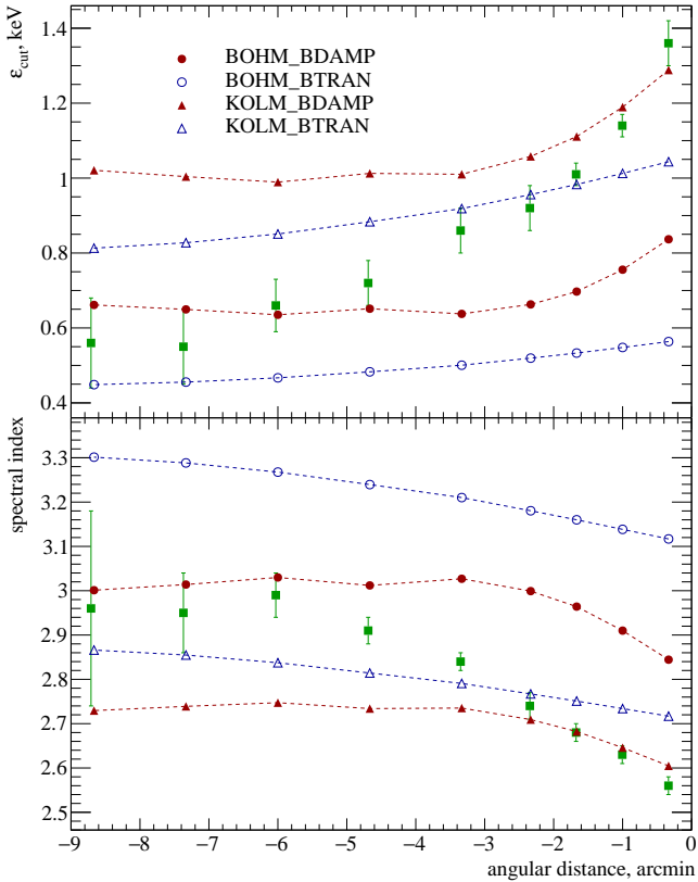
Fig. 6. Simulated projected radial profiles of the X-ray spectral parameters for four different models assuming spherical symmetry. Top panel: cut-off energy and the bottom one shows the spectral index in the 2–10 keV band as a function of the angular distance from the forward shock of the SNR. The distributions are obtained by extracting the spectrum for each region and fitting it with an exponential cut-off power law assuming a photon spectral index of \Gamma = 1.6 ( top panel ) and with a simple power law ( bottom panel ). In both panels, green squares indicate the observational data (Kishishita et al. 2013).
