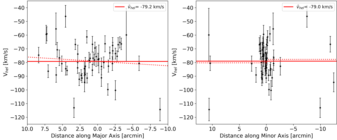
Fig. 6. Line-of-sight velocity distributions of the probable members. Left panel: along the optical major axis, with the systemic velocity (solid line) and the rotational component (dotted line) resulting from MultiNest run using the linear rotation model overplotted; right panel: along the minor axis, with the systemic velocity (solid line) and the rotational component (dotted line) resulting from MultiNest run using the flat rotation model overplotted. As can be seen from both panels the rotational component is negligible.
