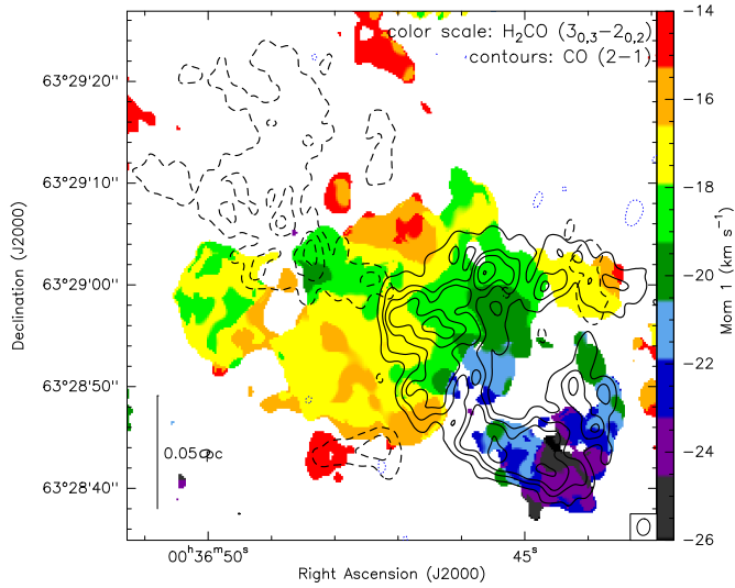
Fig. 7. Contours: CO (2–1) red- (dashed) and blue- (solid) shifted emission at \pm 12 km s ^{-1} from the systemic velocity -17.4 km s ^{-1} . Contour levels are -6, 6, 18, 30, 50, 70 times the rms level 0.04 Jy beam ^{-1} . The synthesized beam located in the bottom-right corner is 1''.66 \times 1''.38 , PA = -8^\circ . Color scale: intensity-weighted averaged velocity (i.e., moment 1) map of H _2 CO 3(0,3)–2(0,2) emission. A scale bar is located in the bottom-left corner.
