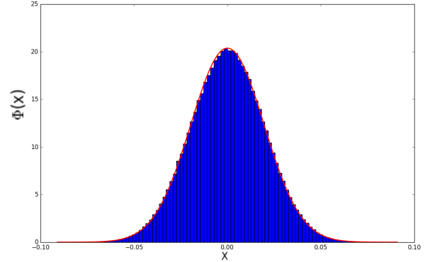
Fig. 4. Histogram of the pixel values from the ALMA data cube (our observations). The blue histogram comes from the pixel values and the red curve is a Gaussian fit. We see that the noise is a perfect Gaussian which does not show any indication of bumps that could be related to the reduction and deconvolution procedures.
