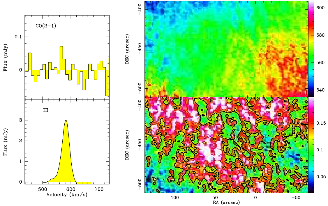
Fig. 5. Left panels: result of the stacking procedure for the CO(2-1) map ( top ) and the HI map ( bottom ). Only spectra with a significant HI detection have been considered (see text), and they have all been shifted to 580 \text{ km s}^{-1} central velocity. Right panels: HI (THINGS) integrated intensity map ( \text{Jy} \times \text{km s}^{-1} , bottom ) in the region of the mosaic observed by ALMA, and the corresponding average velocity ( top ) in \text{km s}^{-1} . The spatial coordinates are in arcsec offset from the galaxy centre ( 13^{\text{h}}37^{\text{m}}00.9^{\text{s}} , -29^{\circ}51'56'' ). The HI beam is 15.2'' \times 11.4'' (VLA NA map from THINGS). The black contour corresponds to \text{NHI} = 10^{21} \text{ cm}^{-2} .
