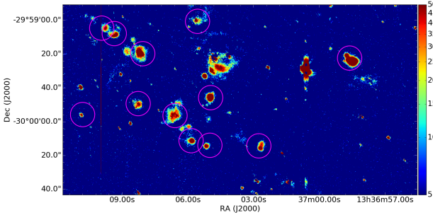
Fig. 3. H\alpha image of the region from Subaru (Koda et al. 2012). The magenta circles show the positions where CO was searched.
