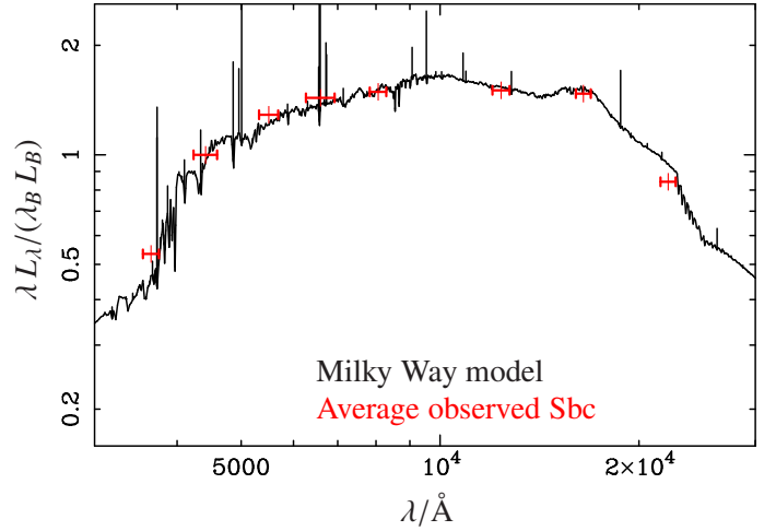
Fig. 5. Near-UV-to-near-IR spectral energy distribution of the 13 Gyr-old Milky Way model (black line), compared with the mean observed fluxes of local Sbc galaxies (red crosses) in the U, B, V, R_c, I_c, J, H and K passbands (see Sects. 7.1 and 7.2 for details). All fluxes were normalized to the B band. The red horizontal segments correspond to the width of the passbands. See also Table 2.
