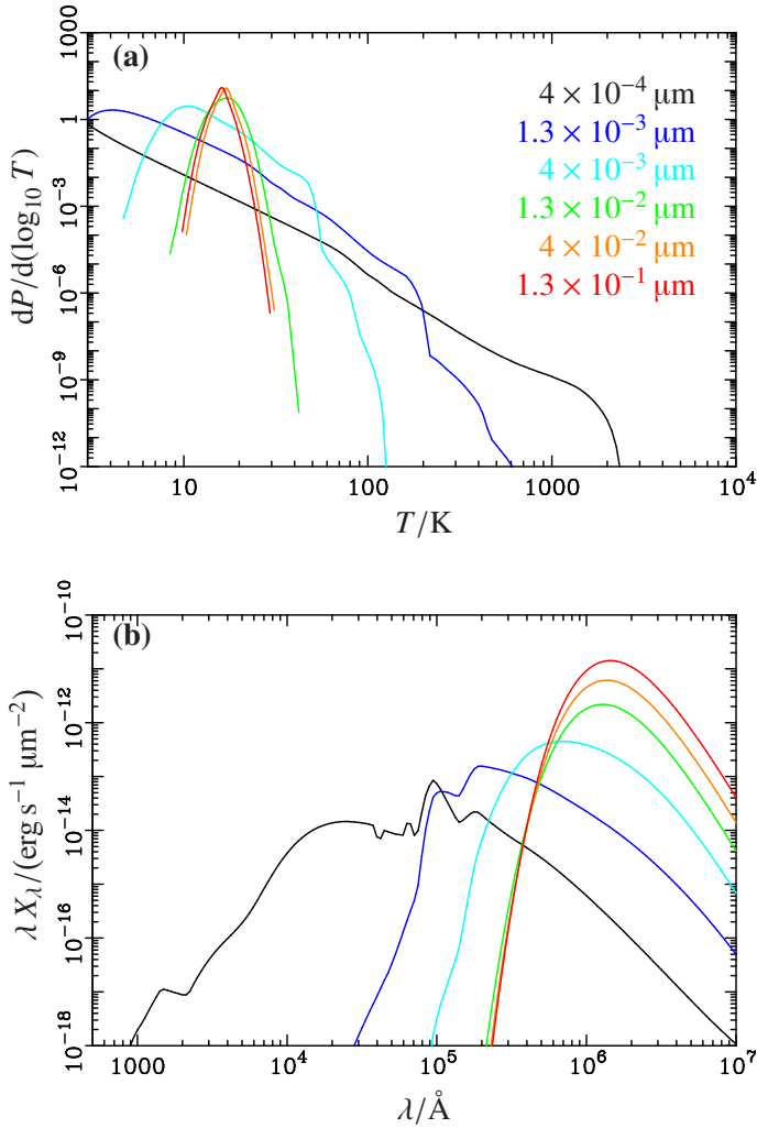
Fig. 9. Panel a: temperature probability distribution of silicate grains in the diffuse medium of the 13 Gyr-old Milky Way model. Grain radii are color coded as indicated on the plot. Panel b: emission spectra of these grains (same color coding for grain radii as in previous subfigure). The quantity X_{\lambda} is the spectral exitance (luminosity per unit surface of the grain).
