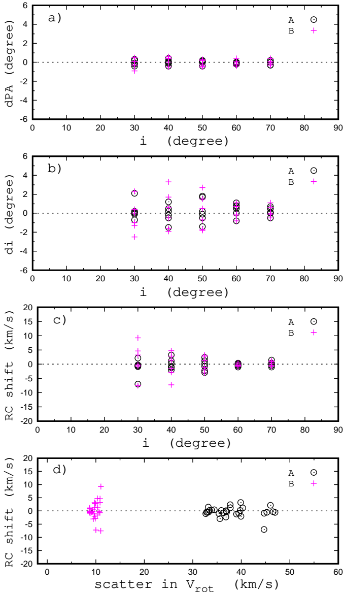
Fig. 3. Panel a): difference between the obtained and the true position angle of the major axis d(PA) as a function of inclination angle for our set of models. Panel b): difference between the obtained and the true inclination angle di as a function of inclination angle. Panel c): mean shift of the obtained rotation curve relative to the true rotation curve as a function of the inclination angle. Panel d): mean shift of the obtained rotation curve as a function of the value of the scatter of the spaxel rotation velocities around the obtained rotation curve. Cases A and B are shown by circles and plus signs, respectively, in each panel.
