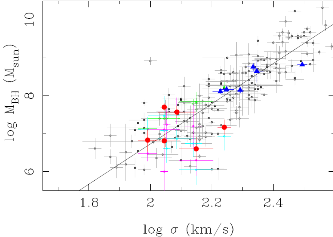
Fig. 21. Location of our galaxies in the M_{\text{BH}}-\sigma relation, compiled by van den Bosch (2016) , represented by the gray points and the fitted line, of slope 5.35. Our galaxies are in red, while in blue are plotted other values recently obtained from the CO line: NGC 1097 ( Onishi et al. 2015 ), NGC 1332 ( Barth et al. 2016 ), NGC 3665 ( Onishi et al. 2017 ), NGC 4429 ( Davis et al. 2018a ), NGC 4526 ( Davis et al. 2013 ), NGC 4697 ( Davis et al. 2017 ). Previous estimations of the BH masses of our sample galaxies are also plotted in green (Table 6), turquoise and pink (Cols. 2 and 3 in Table 7).
