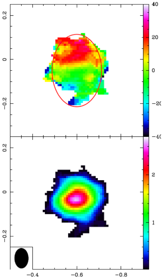
Fig. 7. First moments of the HCO + (4-3) map of NGC 613. The color scale of the intensity at the bottom is in \text{Jy beam}^{-1} \times \text{km s}^{-1} , and the velocity at the top is in \text{km s}^{-1} . The red ellipse at the top indicates the definition of the molecular torus. The RA-Dec scale is in arcsec.
