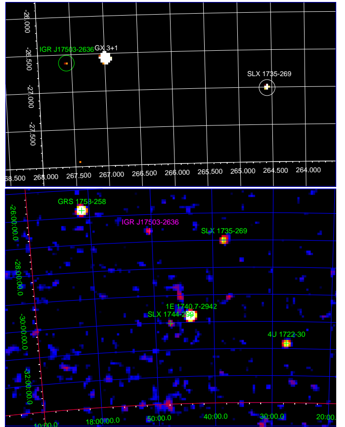
Fig. 1. Zoom of the JEM-X (upper panel) and IBIS/ISGRI (bottom panel) mosaic of the region around IGR J17503–2636 obtained by combining all publicly available data from 2018 August 10 at 15:50 to 2018 August 11 at 18:52. The source is detected at a significance of 7\sigma in the IBIS/ISGRI mosaic and 6\sigma in the JEM-X mosaic.
