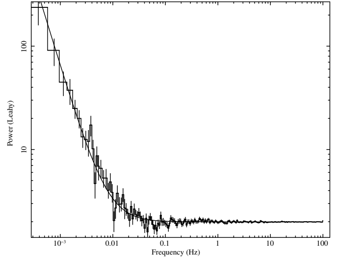
Fig. 4. Power spectral density of the NuSTAR summed light curve in the 3–60 keV energy range binned at 0.005 s. The power spectrum was obtained by averaging 15 segments of 524 288 bins and rebinned geometrically with a factor of 0.05.
