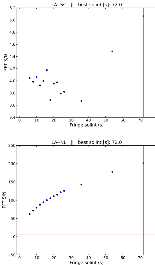
Fig. 3. Example plots of a fringe fit solution interval optimization search based on 7 mm VLBA data (Sect. 6). Los Alamos (LA) is chosen as the reference station for the scan shown. The blue points show the FFT S/N as a function of solution interval, the horizontal red line indicates the S/N cutoff of 5 on each baseline, and the vertical red line shows the smallest solution interval of 72 s needed to reach the S/N cutoff on each baseline for this scan. The top plot shows the baseline to the Saint Croix (SC) station, which has driven the solution interval to higher values until a detection was made when we integrated for 72 s. The bottom plot shows data from the same scan for the baseline to the North Liberty (NL) station, where the source was detected for each solution interval, yielding the expected increase in S/N with the square root of the solution interval.
