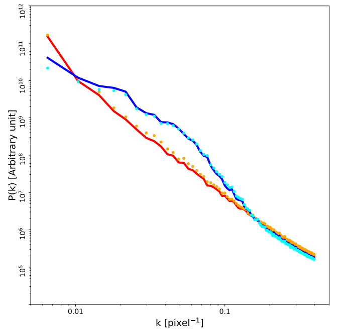
Fig. 12. Spatial power spectrum of the column density. The inter-cloud medium (WNM + LNM) is represented by the orange dotted line (simulation) and the red line (ROHSA). The CNM is shown as a cyan dotted line (simulation) and blue line (ROHSA).
