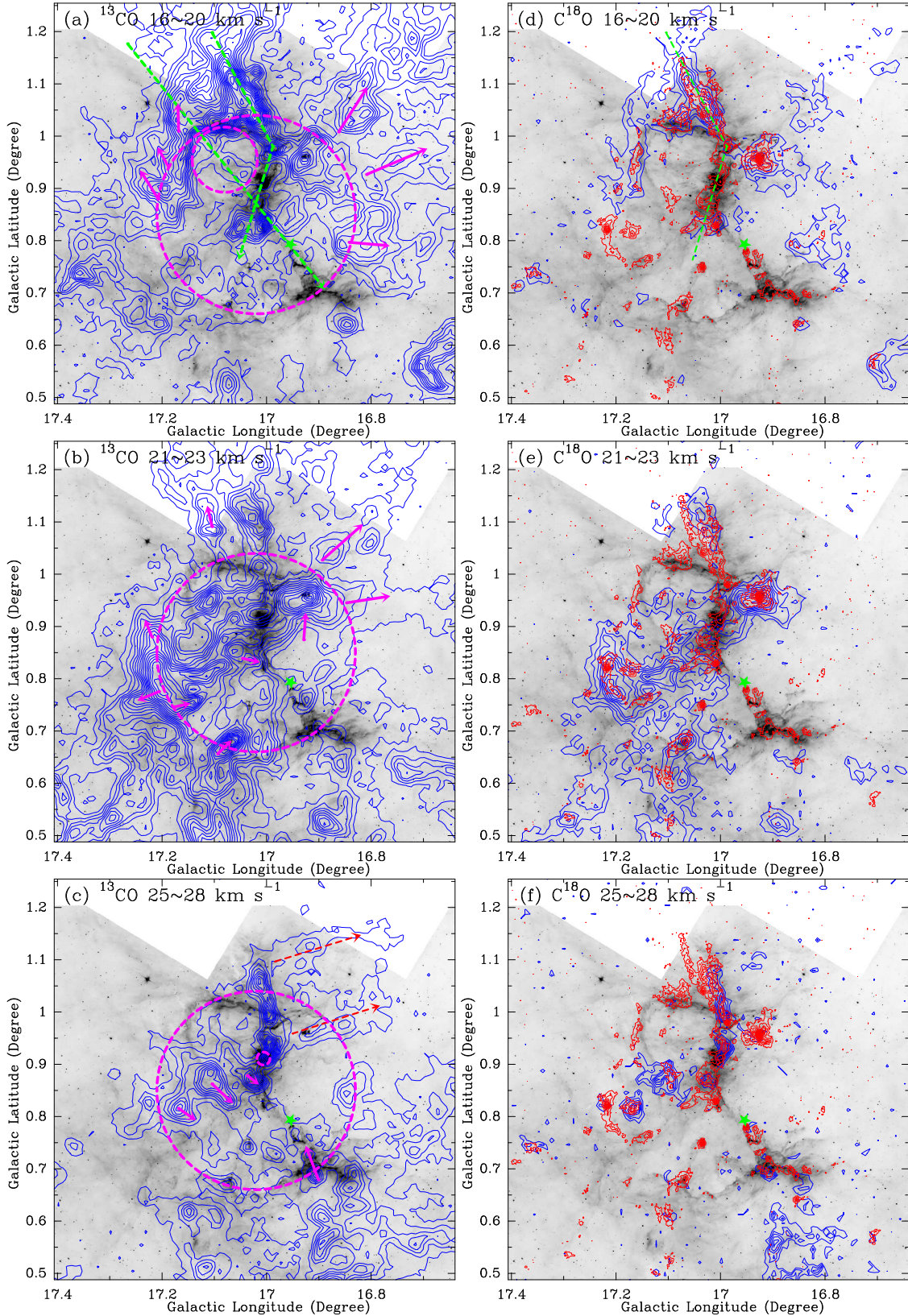
Fig. 5. Panels a–c : ^{13}\text{CO} integrated intensity maps (blue contours) superimposed on the Spitzer -IRAC 8\mu\text{m} emission (gray). The integrated-velocity ranges are shown on top of each image. The pink arrows mark the pillars, while the red dashed arrows indicate two gas flows. The blue contour levels start from 0.2\text{ K km s}^{-1} ( 5\sigma ) in a step of 1.6\text{ K km s}^{-1} . The pink dashed circles represent M 16, N19, and RCW165. The green star marks the NGC 6611 cluster ionizing M 16. Panels d–f : \text{C}^{18}\text{O} integrated intensity images overlaid with the ATLASGAL 870\mu\text{m} (red contours) and 8\mu\text{m} emission (gray). The blue contour levels start from 0.15\text{ K km s}^{-1} ( 5\sigma ) in a step of 0.75\text{ K km s}^{-1} , while the red contour levels start from 0.06\text{ Jy beam}^{-1} ( 3\sigma ) in a step of 0.3\text{ Jy beam}^{-1} . The green dashed lines mark the directions of position–velocity diagrams in Fig. 10.
