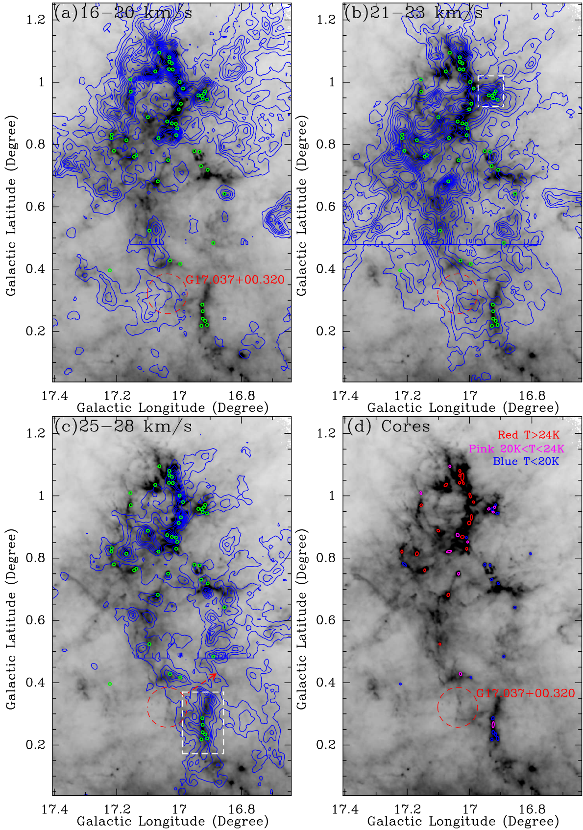
Fig. 6. Panels a–c: the ^{13}\text{CO } J=1-0 emission in blue contours overlaid on the Herschel 250 \mu\text{m} emission in grayscale. The integrated-velocity ranges are shown on top of each image. The green circles represent the 870 \mu\text{m} dust cores, while the red dashed circle shows the position and size of G17.037+00.320 H II region from Anderson et al. (2014). The red arrow may present the shock direction. The two white dashed boxes indicate the compact region with six dust cores. Panel d: the ellipses also mark the positions, sizes, and position angles of the 870 \mu\text{m} dust cores, which are given in Table 1. The different colors mark the cores with different temperatures ( T ). If T > 24\text{K} , the cores are marked in red, for 10\text{K} < T < 24\text{K} and T < 10\text{K} in pink and blue, respectively.
