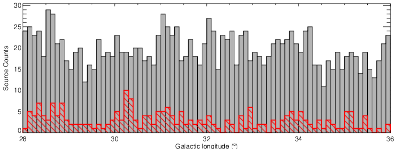
Fig. 23. Distribution of GLOSTAR radio sources as a function of Galactic longitude. The whole catalog is shown as the gray histogram while the sources identified as H II regions are shown as the hatched red histogram. The bin size used for both distributions is 0.1^\circ .
