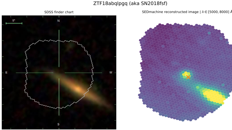
Fig. 5. Illustration of the SEDM field of view; ZTF18abqlpgq. Left: RGB SDSS image centered at the target (ZTF18abqlpgq) location. The gray line represents the SEDM footprint for this target. Right: integrated 2D image of the corresponding SEDM 3D-cube. The orange cross shows the expected target location used as first guess for the automatic PSF extraction. We clearly see the point source near its expected position as well as the host galaxy.
