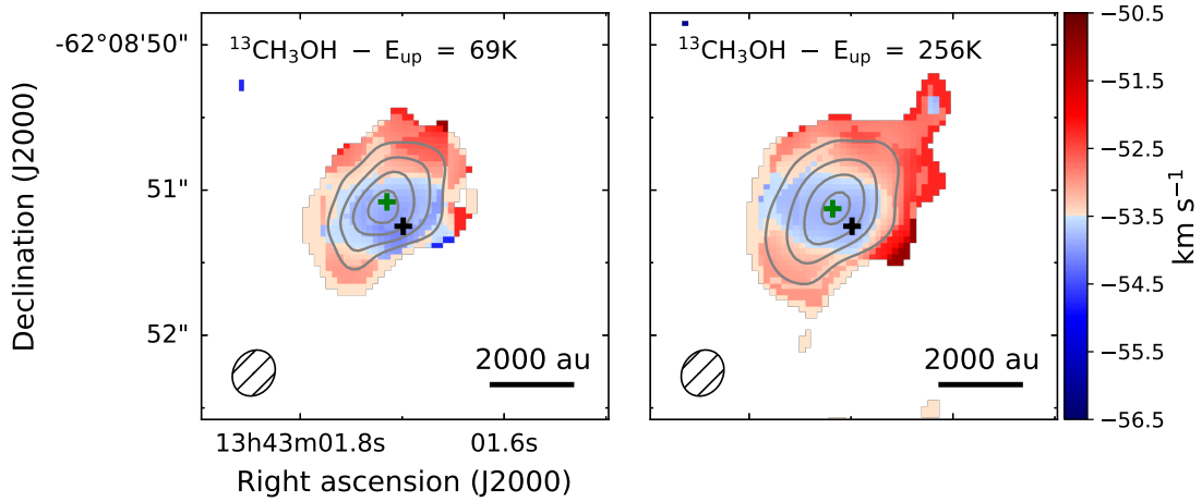
Fig. D.1. Same as Fig. 3 for 13 CH 3 OH lines at 256.1716 GHz (left) and 253.6895 GHz (right). Contours start at 9σ and are in steps of 6σ and 12σ, with σ = 6.27 × 10 -3 and 6.87 × 10 -3 Jy beam -1 km s -1 , for the left and right panels, respectively.
