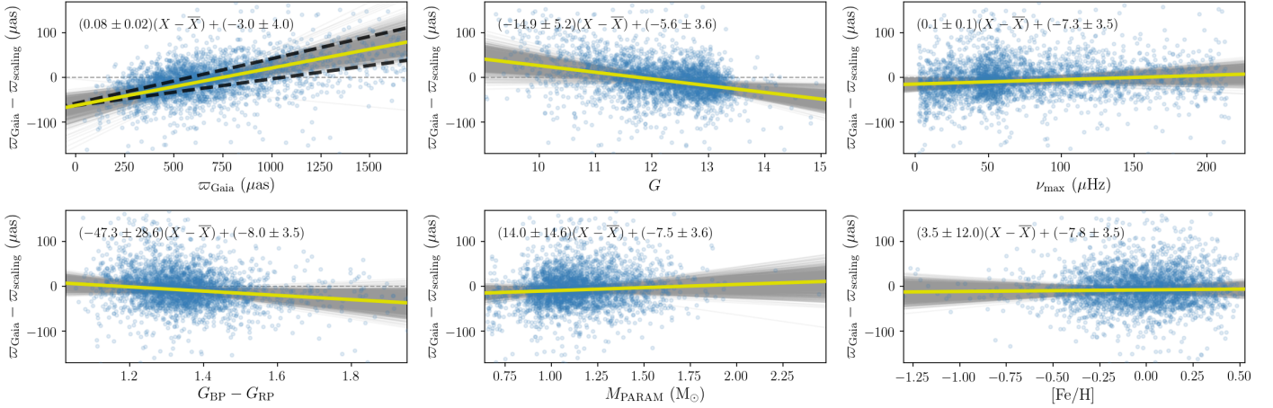
Fig. 2. Parallax difference \varpi_{\text{Gaia}} - \varpi_{\text{seismo}} for RGB stars, with the asteroseismic parallax derived from raw scaling relations, as a function of \varpi_{\text{Gaia}} , G , \nu_{\text{max}} , G_{\text{BP}} - G_{\text{RP}} , M_{\text{PARAM}} , and [Fe/H]. The distribution of the N realisations of the RANSAC algorithm is indicated by the grey-shaded region and the yellow line displays the average linear fit, for which the relation is given at the top of each subplot. The values of \bar{X} for RGB stars are given in Table 1. The summary statistics are: (\Delta\varpi)_{\text{m}} = -6.2 \pm 1.3 \mu\text{as} , (\Delta\varpi)_{\text{w}} = -7.9 \pm 0.8 \mu\text{as} , and z = 0.89 . The black dashed lines correspond to the average linear fits when a \pm 100 K shift in T_{\text{eff}} is applied.
