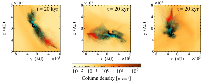
Fig. 6. Column density in three planes of coordinate system (width: 1.6 \times 10^4 au; left : yz -plane, middle : zx -plane, right : xy -plane) at time t = 20 \times 10^3 yr after formation of primary A. The colored dots illustrate the origin and dynamics of accreting gas of the individual sinks. Black (cyan, red) dots represent particles that are located within a distance of 30 au from the primary A (B, C) at t = 90 \times 10^3 yr.
