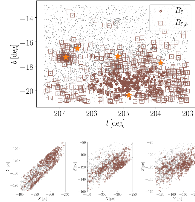
Fig. 8. Top panel: sky distribution of the sources belonging to group B_{5,b} (brown empty squares), group B_5 (brown dots), and all the sources in the Belt region defined in the text (grey dots). The orange stars mark the position of \sigma Ori, \zeta Ori, \epsilon Ori, \eta Ori, and \delta Ori. Bottom panels: distribution in 3D galactic co-ordinates of group B_{5,b} (brown squares), and of all the sources belonging to the Belt region (grey dots).
