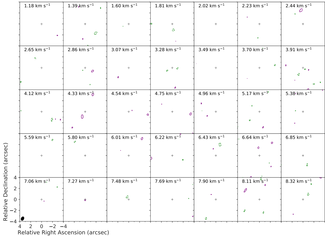
Fig. B.1. Residual (data–model) HCO + ( top ) and H 13 CO + ( bottom ) channel maps at a velocity resolution of 0.21 km s -1 . The rms is 0.016 Jy beam -1 km s -1 channel -1 the purple and green contours are ±3, 5, 7σ, respectively.
