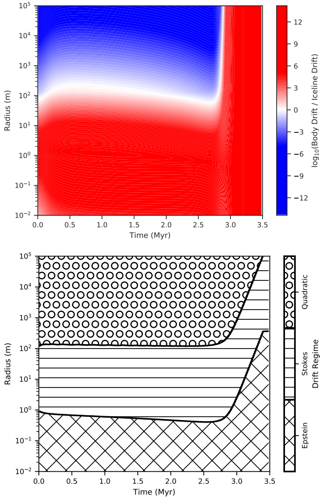
Fig. 7. Drift velocity compared to water snow line velocity ( top panel ) and drag regime ( bottom panel ) in an irradiated disk with photoevaporation. All the bodies with sizes in the red area in the top panel cross the snowline, since they drift faster than it moves toward the central star. The snowline is determined using tabulated values for the temperature and pressure. After approximately 2.4 Myr, the snowline position starts to move away from the star, due to the disks dispersal. Thus, the ratio of the body's drift speed to the snowline speed is negative and the log in the top panel is no longer defined and the ratio is set to a value of 12 to indicate that all the bodies will cross the snowline in that phase. In order to smooth out numerical artifacts, we applied a Gaussian filter in horizontal direction.
