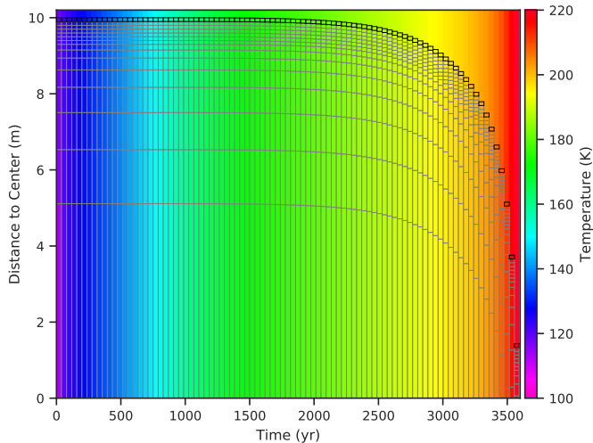
Fig. 13. Interior temperature of an initially ten-meter-sized body covered by a 10 cm thick dust mantle. The number of layers is reduced to 15 compared to nominal runs for better visibility and 60 timesteps are merged into one block. The uppermost, dark framed layer shows the dust mantle. Outside the body, the local disk temperature is plotted. A radial temperature gradient is only barely visible.
