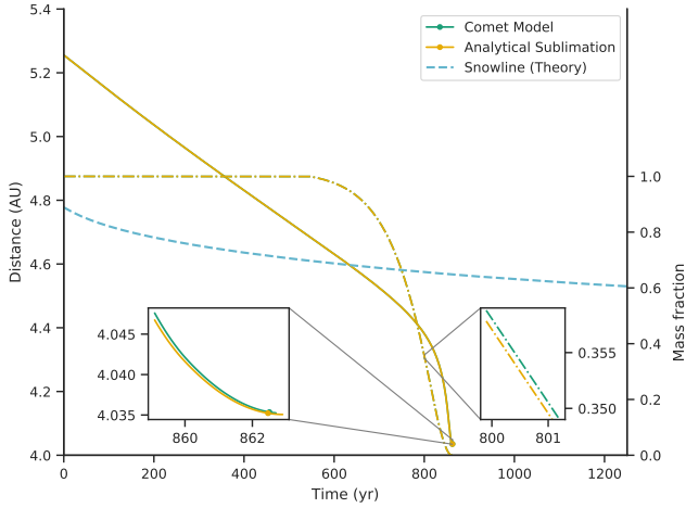
Fig. 4. Comparison of the comet model solving the internal structure and the analytical solution (Eq. (12)) for ten-meter-sized bodies. The solid lines show the distance to the star (left axis) with dots representing the locations where the bodies shrank to a size of 10 cm while the dash-dotted lines show the remaining mass fraction (right axis). The lines of the two different model solutions are essentially indistinguishable. The initial position is 10% above the snowline location at time zero in the nominal disk. The barely visible kink in the mass fractions at 600 yr is due to reaching the threshold temperature of 150 K, where the sublimation models are started.
