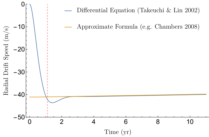
Fig. A.1. Radial drift speed comparison between the approximate Eq. (8) and the numerical solution to the differential equations. The radius is 1 m, the initial location is at 2 AU, temperature and midplane density are constant over the disk and set to 140 K and 2.5 \times 10^{10} \text{ g cm}^{-3} . Initially the body moves with Keplerian speed in azimuthal direction and no radial velocity. The dashed, vertical line marks the stopping time.
