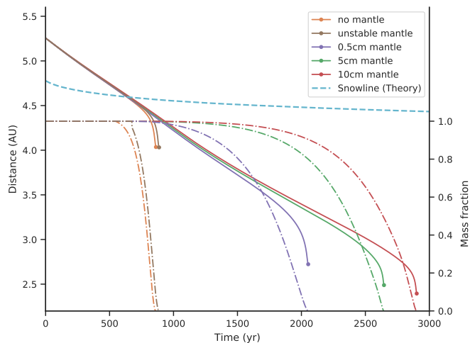
Fig. 11. Sublimation comparison of a ten-meter-sized bodies with different dust mantle thicknesses and removal processes. The legend is ordered in increasing sublimation time. The smooth line marks the location of the body in time (left axis), while the dots at the end of the line indicate shrinking to a radius of 10 cm as in Figs. 8 and 12. The dash-dotted lines indicate the mass fraction compared to the initial mass of the same colored case (right axis). The kink that is visible in the mass fraction of the unstable (initially 5 cm thick) mantle stems from the mantle breaking up at that point in time.
