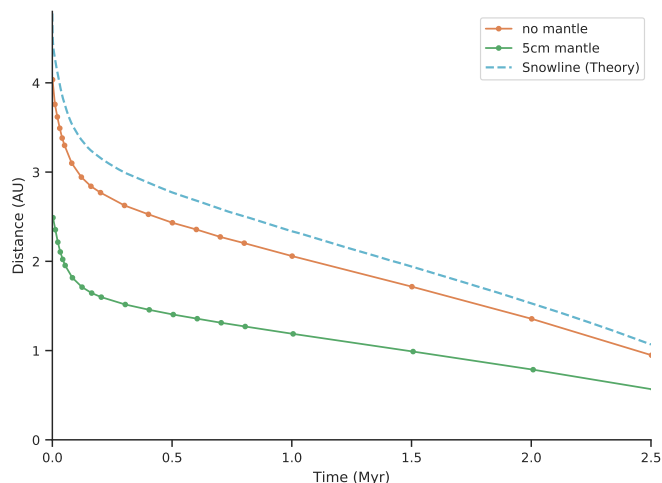
Fig. 12. Locations of complete disintegration in the nominal disk of initially ten-meter-sized bodies with and without a dust mantle. The classical water ice line (snowline) in the disk is indicated for reference.
