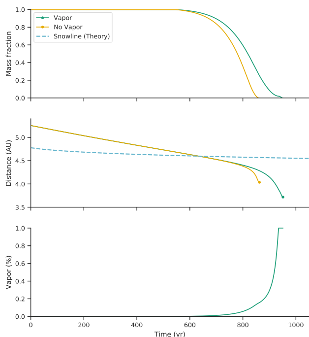
Fig. 16. Evolution of a ten-meter-sized body in the nominal disk calculated with the analytical surface ablation model, with and without water vapor pressure. The water vapor increases exponentially depending on the local disk temperature up to a maximum of one percent of the local pressure.
