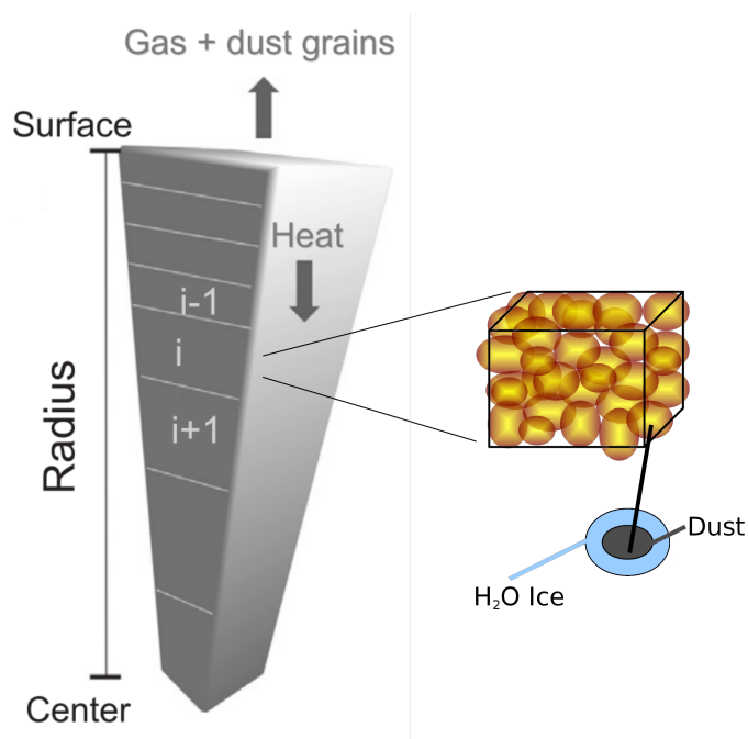
Fig. 1. Schematic view of structure model. Adapted from Marboeuf & Schmitt (2014) .
