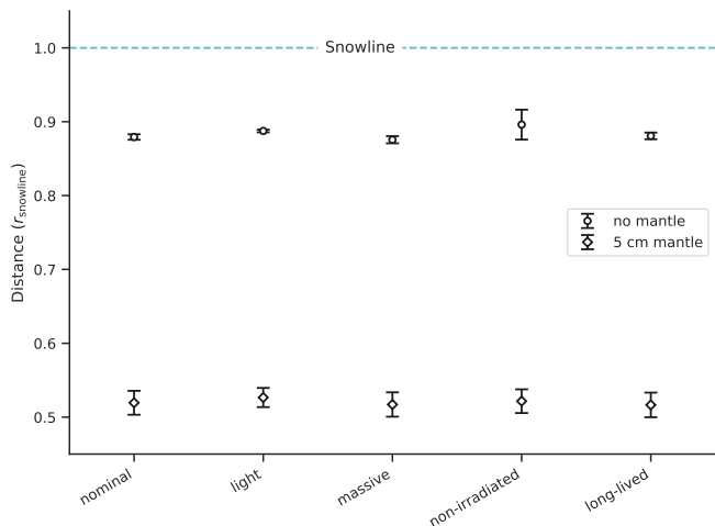
Fig. 10. Mean relative locations of complete disintegration in different disks for initially ten-meter-sized bodies with and without constant dust mantles. As in the bottom panel of Fig. 8, the distance from the central star is measured in units of snowline positions (snowline location at 1, star at 0). The mean over the calculations at different times is taken and the 1\sigma error is indicated. Refer to the text for the different disk properties.
