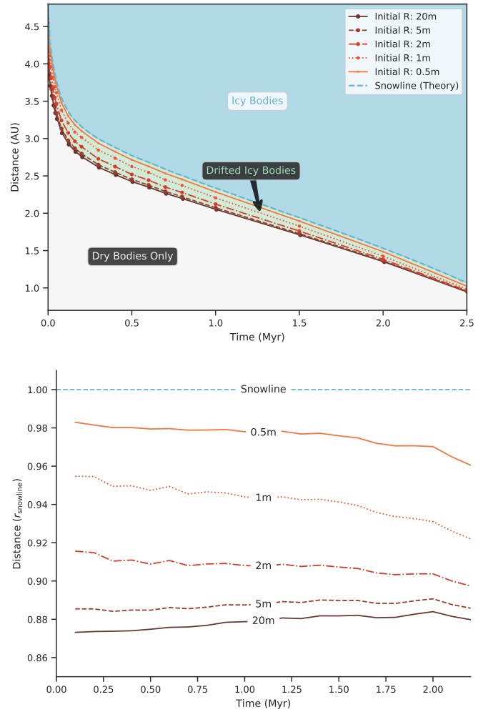
Fig. 8. Comparison of locations of complete disintegration of different sized bodies without a dust mantle. In the top panel , the distance to the star is measured in AU and the dots represent the locations where the body shrank to a size of 10 cm. The dashed, cyan line indicates the evolving position of the P - T tabulated snowline, and the regions where only icy solid bodies, only water depleted solid bodies, and the region that is injected with drifting icy bodies are colored and labeled. In the bottom panel , the same data is shown but measured in units of the evolving, tabulated snowline position (1 corresponds to the snowline position, 0 to the central star).
