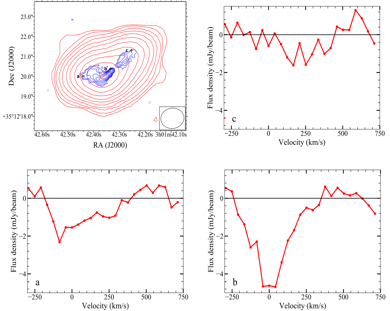
Fig. 2. Top left: VLA continuum map of B2 0258+35 (beam size: 1.13'' \times 0.98'' ; red contours). The contour levels start from 1 \text{ mJy beam}^{-1} ( 3\sigma ) and increase by a factor of two. The 3\sigma negative contours are shown in grey and the beam is shown in the bottom right corner of the image. The regions from which the H I absorption spectra are extracted are labelled. The 22 GHz VLA map (by Giroletti et al. 2005 , beam size: 0.12'' \times 0.12'' ) is overlaid in blue contours to show the underlying continuum structure. These contours start from 325 \mu\text{Jy beam}^{-1} ( 5\sigma ) and increase by a factor of two. Bottom left, bottom right, and top right: absorption spectra extracted from the regions that are marked are in black in the continuum map. The spectra have been Hanning-smoothed and resampled to a velocity resolution of \sim 42 \text{ km s}^{-1} .
