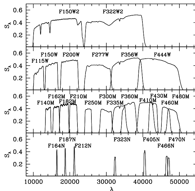
Fig. 1. Total throughput as a function of wavelength \lambda (in Å) for the 27 NIRCcam filters considered in this work. From top to bottom: we show extra wide-, wide-, medium-, and narrow-band filters.
