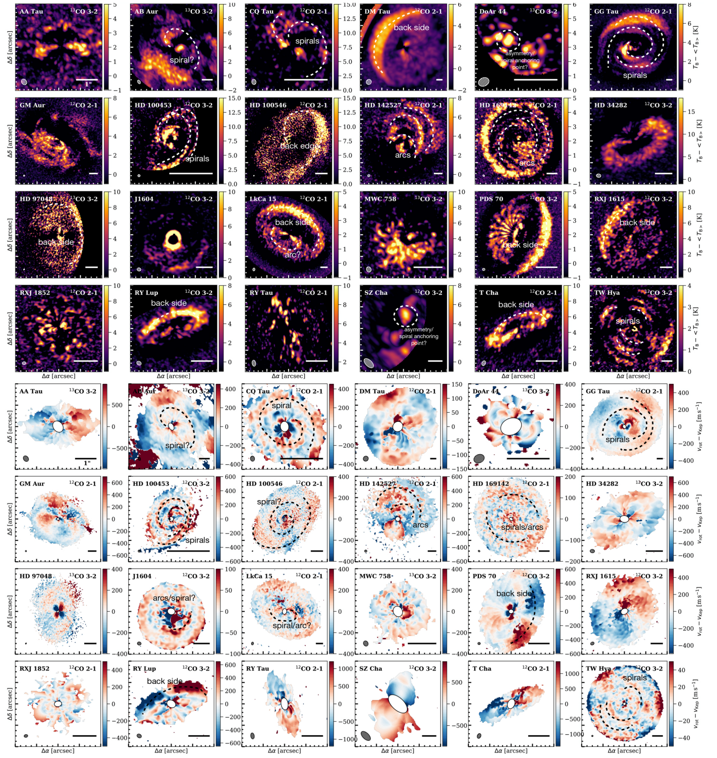
Fig. B.1. Brightness temperature (top) and rotation velocity (bottom) residuals for the main lines used in this analysis and for a thick disc geometry. The circle and bar in the bottom left and bottom right corner of each panel indicate the beam and a 1'' scale, respectively. Some features are annotated.
