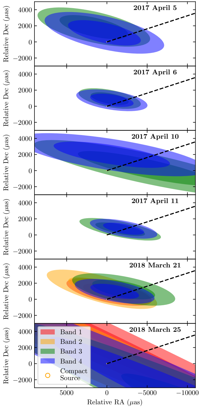
Fig. 4. Estimated two-dimensional 68% and 95% regions of the centroid position offset in M87* for the 2017 and 2018 datasets. The dashed black line at 288° east of north represents the direction of the mas-scale jet.
